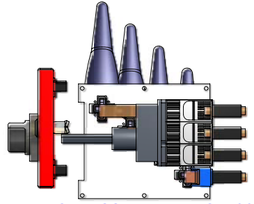
GA-MCCB-LH1x1-NSX100-N-16-TMD 3P-ROT-Fix-FAP-T5-Out
